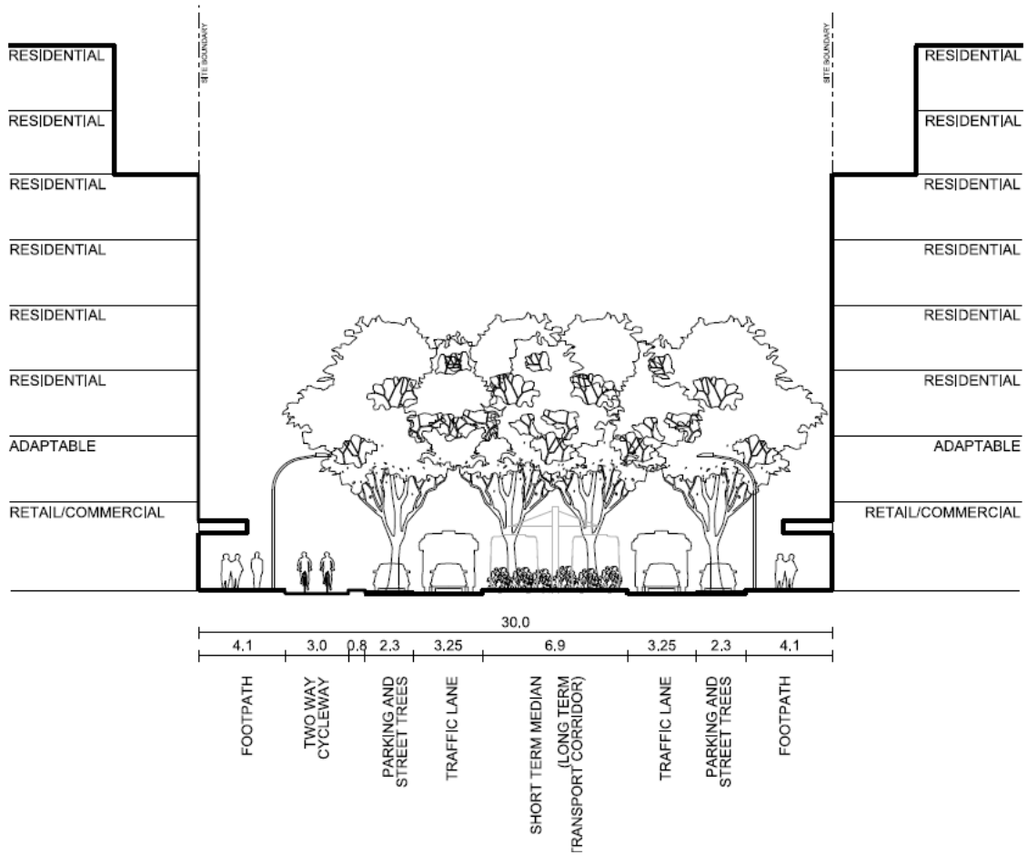
Figure 5.xx: Section A – Transport Corridor Typical Section (short term arrangement) – 30m (Gadigal Avenue)
