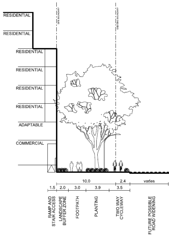
Figure 5.xx: Section J - Landscaped Setback Typical Section (Lachlan Street)
