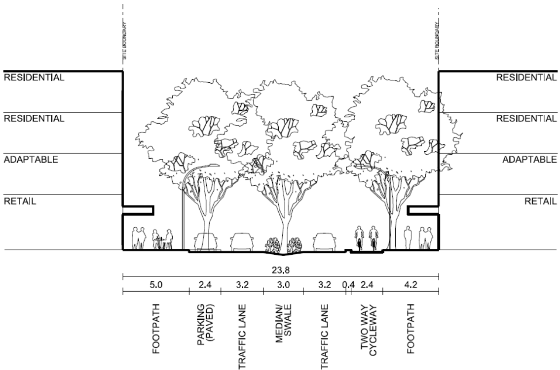
Figure 5.xx: Section B – Main Street Typical Section – 23.8m (Archibald Avenue)
