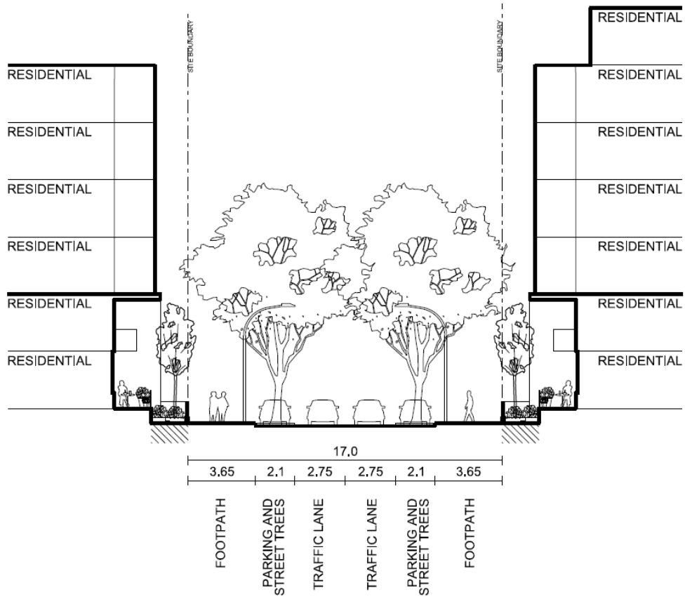
Figure 5.xx: Section E – Local Street Type 2 Typical Section – 17m (Reed Street)
