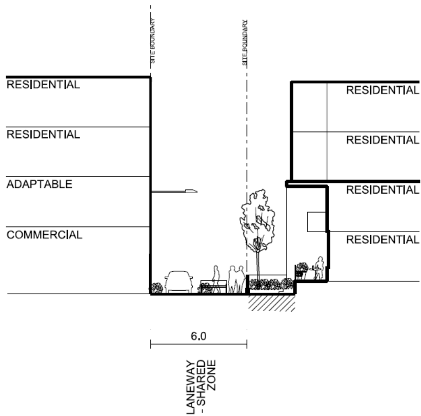
Figure 5.xx: Section G – Laneway - Shared Zone Typical Section – 6m (Hatter Lane)
