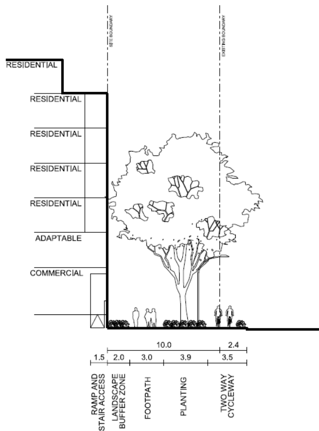
Figure 5.xx: Section K - Landscaped Setback Typical Section (O'Dea Avenue)
