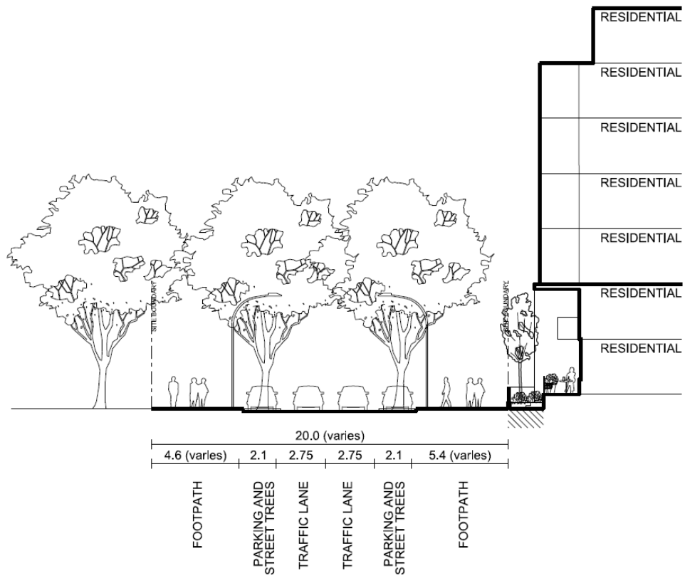
Figure 5.xx: Section D – Local Street Type 1 Typical Section – 20m (Sam Sing Street north)
