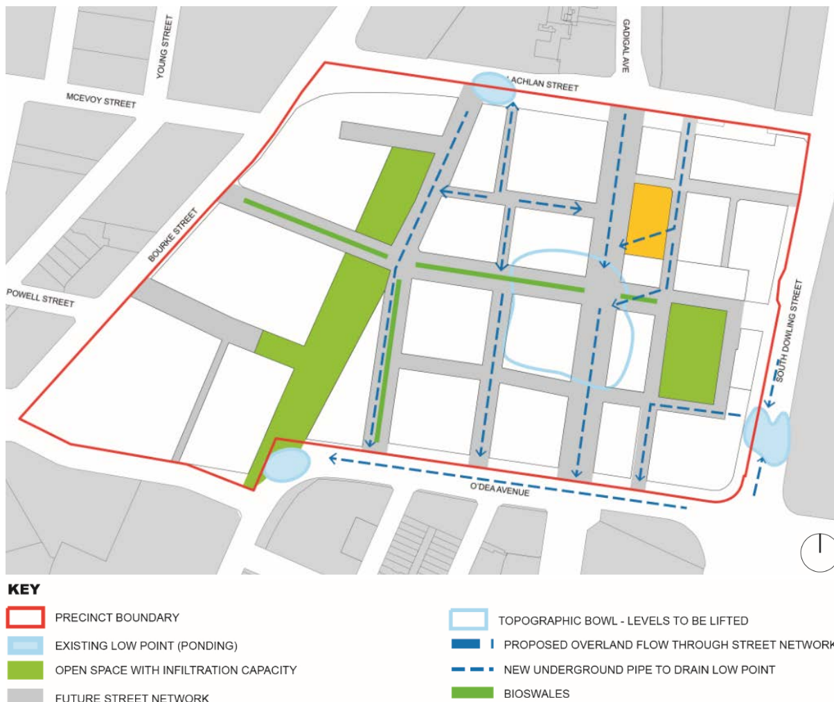
Figure 5.xx: Lachlan Precinct Stormwater Management
