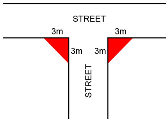
Figure 5.xx: Minimum chamfered setback
