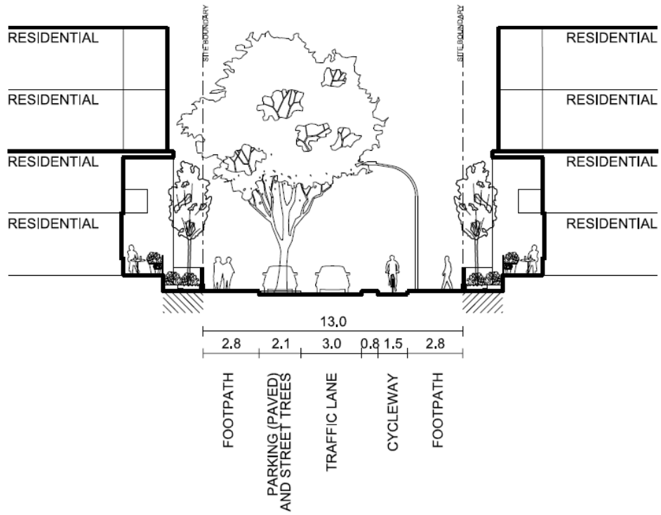
Figure 5.xx: Section F – Local Street Type 3 Typical Section – 13m (Hatbox Place)
