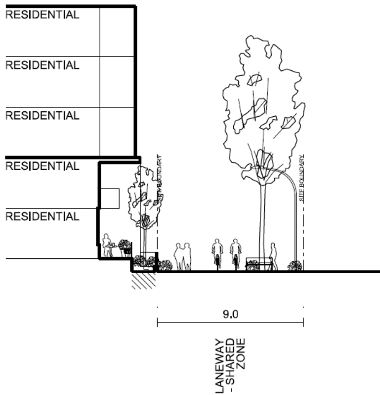
Figure 5.xx: Section I – Laneway - Pedestrian and Cycle Only Typical Section – 9m
