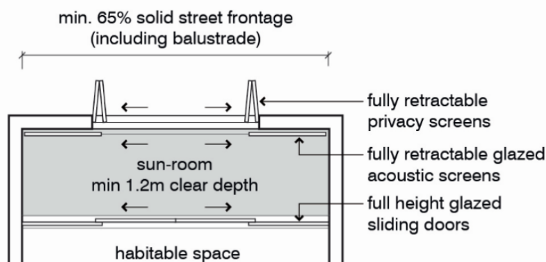
Figure 5.xx: Acoustic and visual privacy treatment for residential units with good access to daylight
