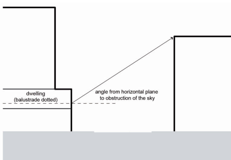
Figure 5.xx: Angle from horizontal plane to obstruction of the sky
