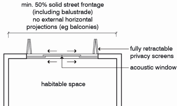
Figure 5.xx: Acoustic and visual privacy treatment for residential units with limited access to daylight
